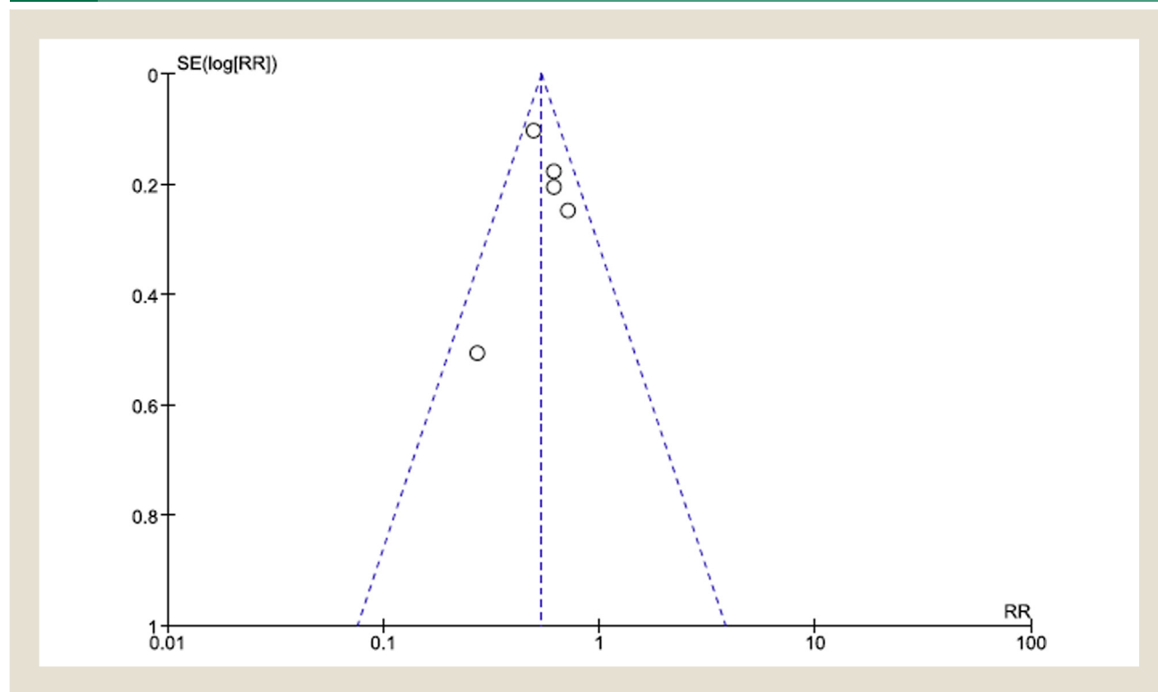
Figure 6 Funnel Plot
